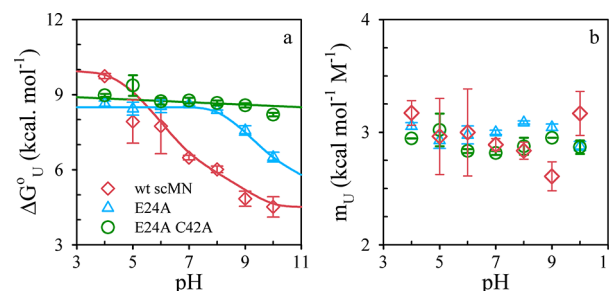
Figure 3. pH dependence of thermodynamic parameters governing the unfolding of wt scMN, E24A, and E24A/C42A (green \circ ). Panels a and b show the values of the thermodynamic parameters \Delta G_{\text{U}}^{\text{o}} and m_{\text{U}} , respectively, obtained by analyzing the equilibrium unfolding transitions using a two-state \text{N} \leftrightarrow \text{U} model. 37 The solid lines through the parameters for wt scMN were drawn using eq 1. The solid lines through the parameters for mutants E24A and E24A/C42A were drawn by inspection only. Error bars, wherever shown, represent the spreads of the measurements taken in at least two independent experiments.
